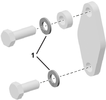
Fig. 2 Parts requirement for inspection - 914 (Series) and 912i (Series)
