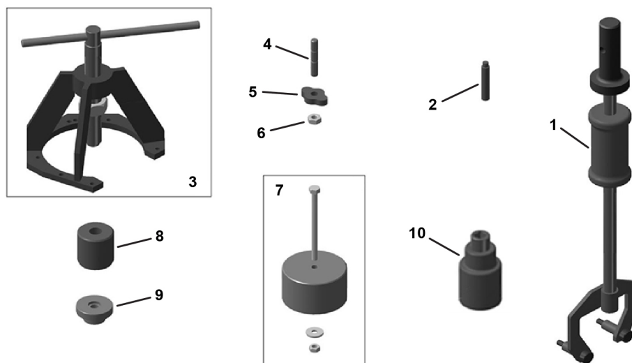
Fig. 6 Special tools
