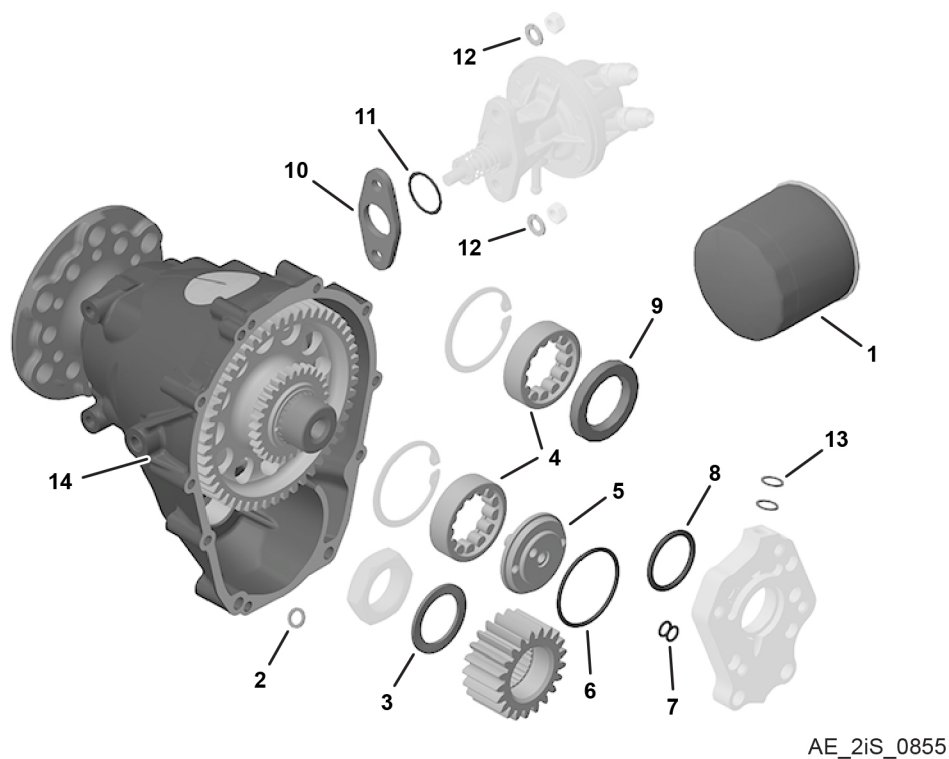
Fig. 3 Parts requirement for gearbox replacement - 912 (Series)
